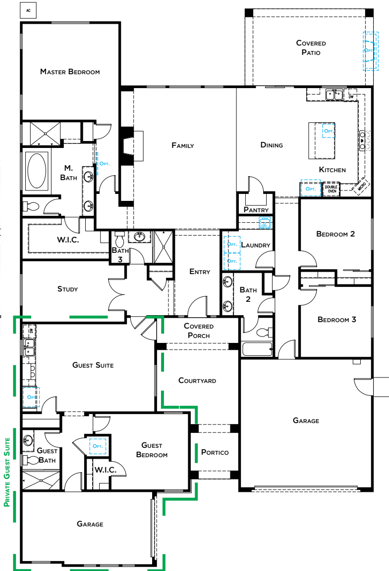
4-CAR GARAGE OPTION
