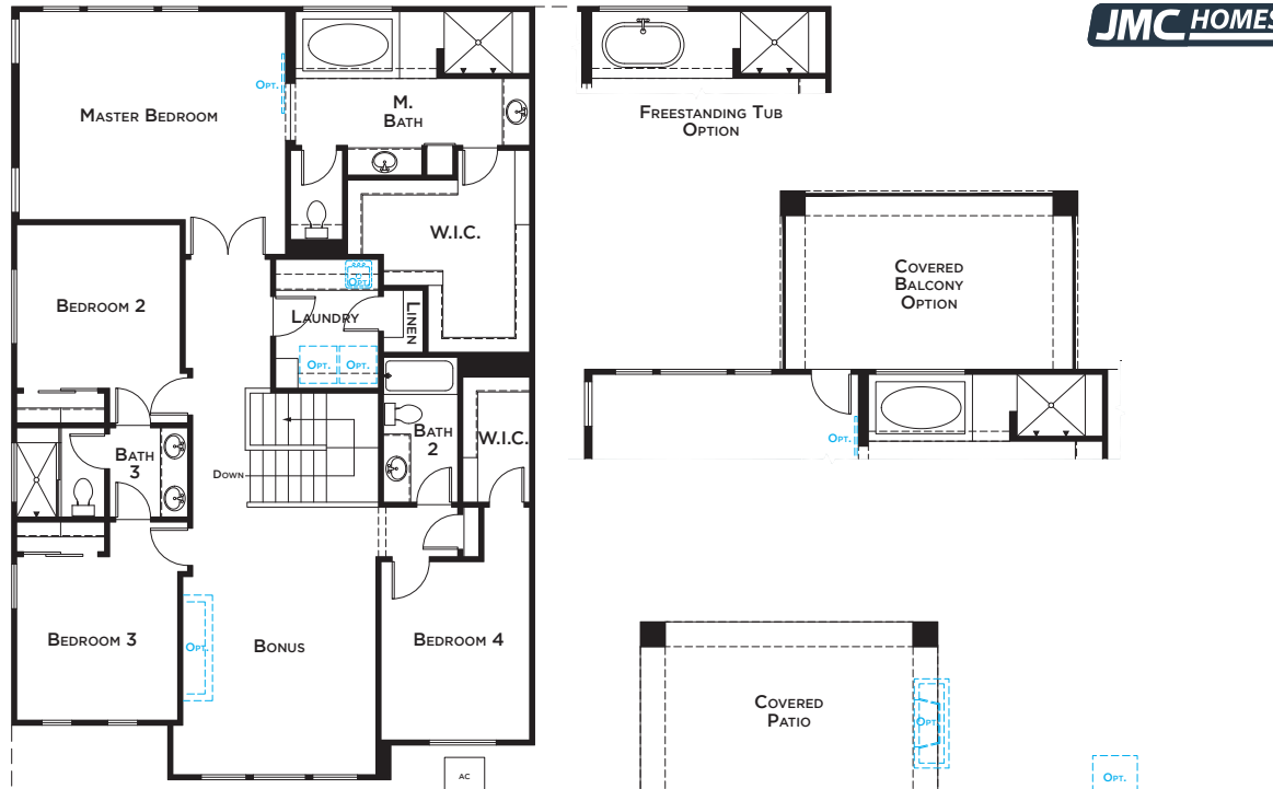
SECOND FLOOR
